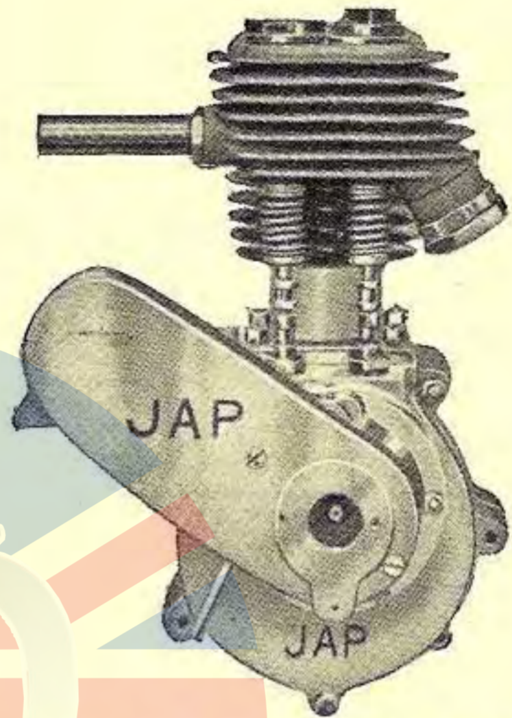
200 c/c. Soupapes Latérales " STANDARD "
