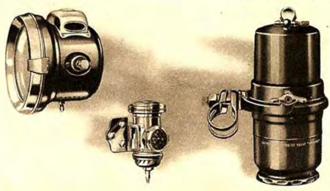
Lucas acetylene lighting set No. 420
