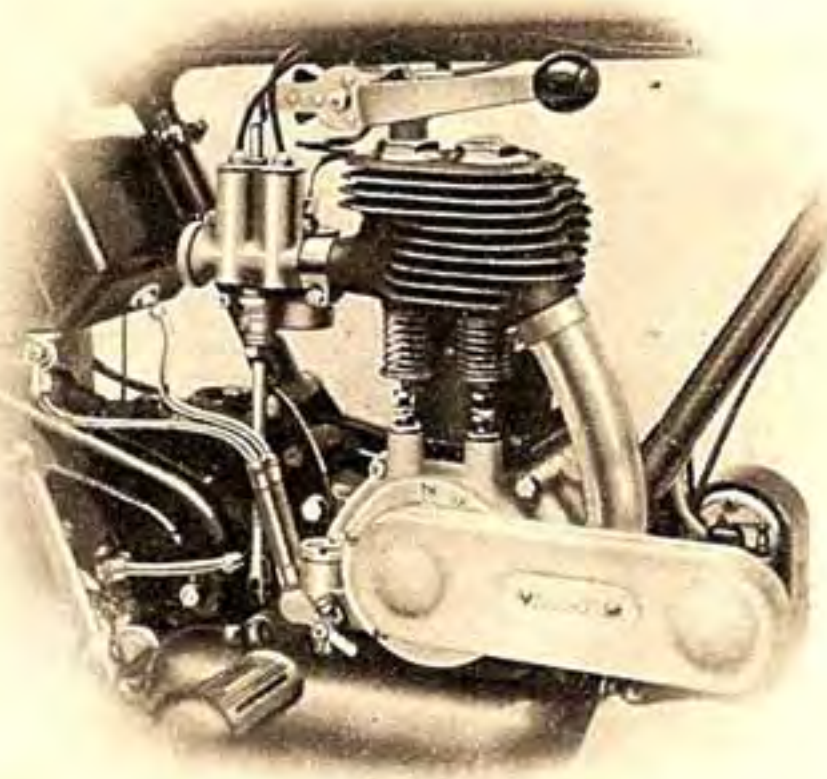
The power unit of the 4.94 h.p. Model N.L.
